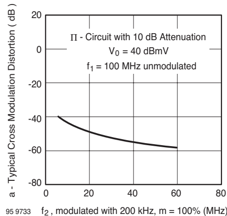
Figure 3. Typ. Cross Modulation Distortion vs. Frequency f_2
