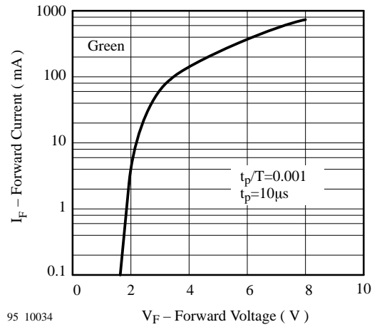
Figure 15. Forward Current vs. Forward Voltage
