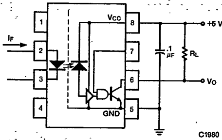
Fig. 3. Input-Output Schematic
