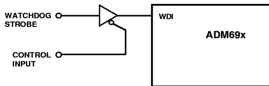
Figure 21a. Programming the Watchdog Input
