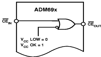
Figure 5. Chip Enable Gating
