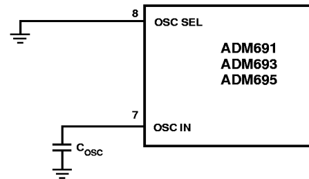
Figure 4b. External Capacitor
