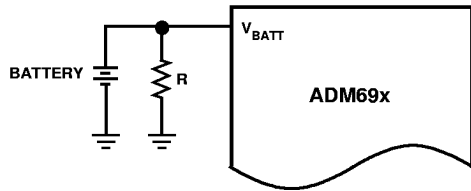
Figure 22b. Preventing Spurious RESETS During Battery Replacement
