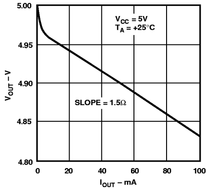
Figure 8. V_{OUT} vs. I_{OUT} Normal Operation
