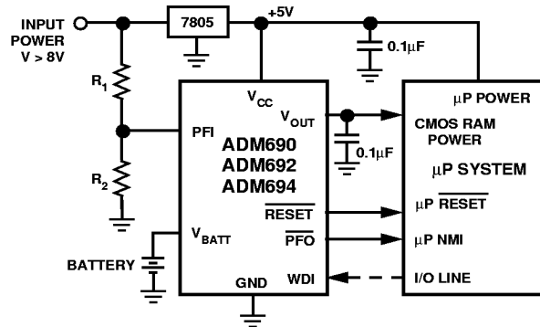
Figure 23b. ADM690/ADM692/ADM694 Typical Application Circuit B
