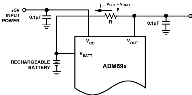
Figure 18. Rechargeable Battery
