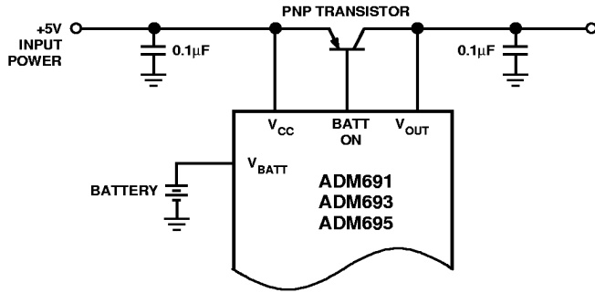
Figure 17. Increasing the Drive Current
