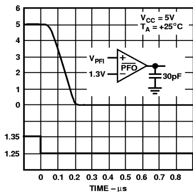
Figure 14. Power Fail Comparator Response Time
