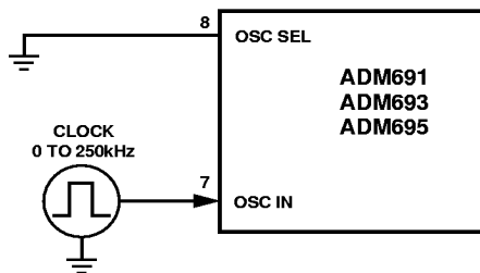
Figure 4a. External Clock Source
