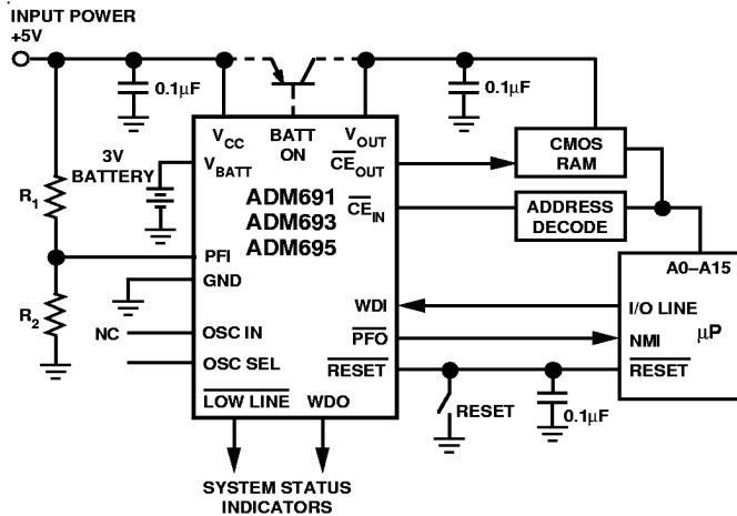
Figure 24. ADM691/ADM693/ADM695 Typical Application
