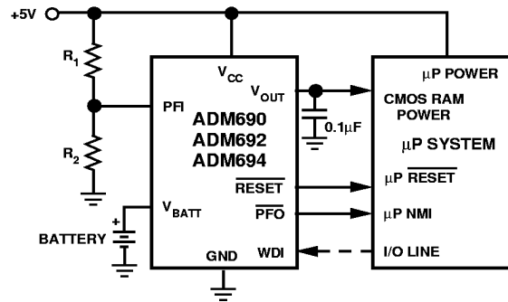
Figure 23a. ADM690/ADM692/ADM694 Typical Application Circuit A
