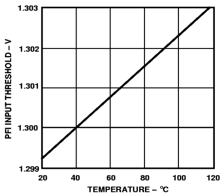
Figure 11. PFI Input Threshold vs. Temperature
