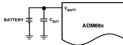
Figure 22a. Preventing Spurious RESETS During Battery Replacement
