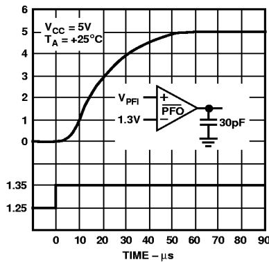
Figure 15. Power Fail Comparator Response Time
