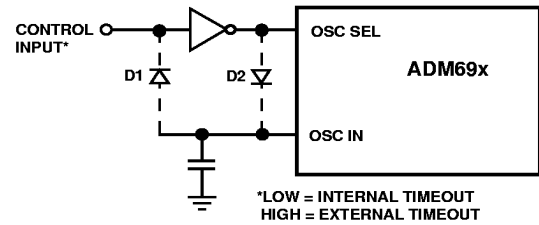
Figure 21b. Programming the Watchdog Input
