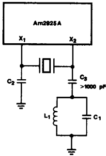
Figure 2. Connections for Frequencies above 20 MHz
