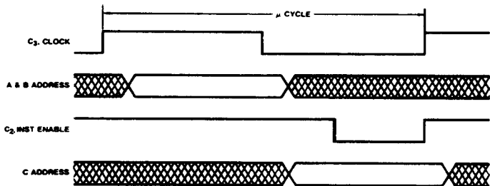
Figure 11. Am2903A Three-Address Operation
