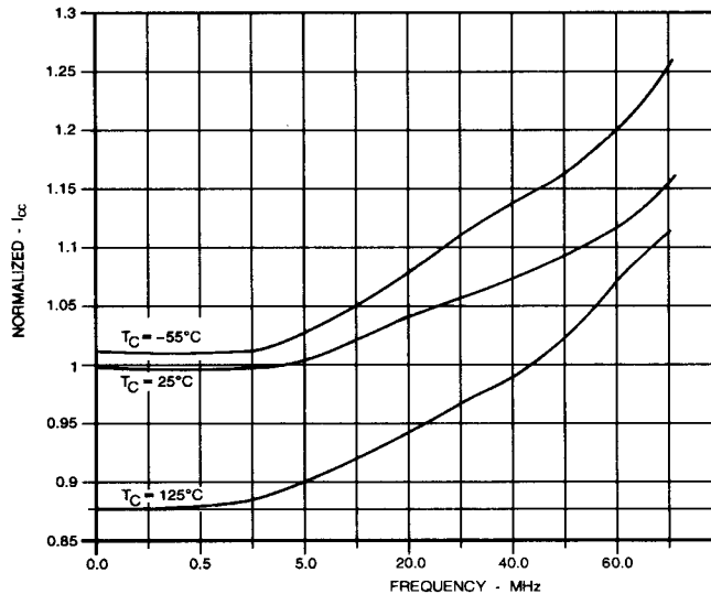
Figure 14. Am2925A I_{CC} Normalized vs Frequency ( V_{CC} = 5.5 V)
