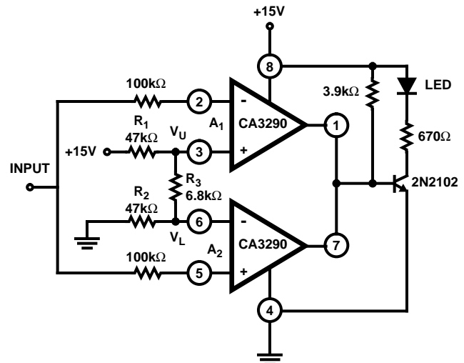
FIGURE 7. WINDOW COMPARATOR
