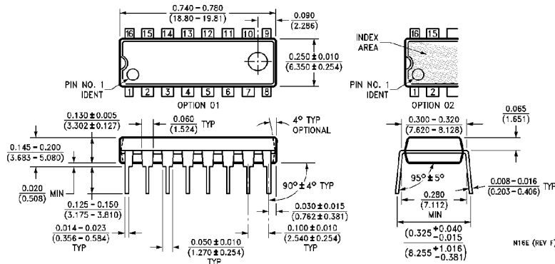
Molded Dual-In-Line Package (N) Order Number CD4020BMN, CD4020BCN, CD4040BMN, CD4040BCN, CD4060BMN or CD4060BCN NS Package Number N16E
