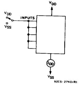
Fig. 12 - Quiescent-device-current test circuit.
