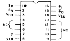
92CS-24478R2 NC - NO CONNECTION
