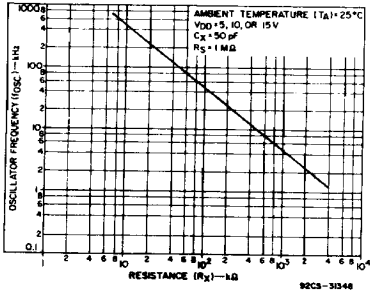
Fig. 10 - Typical RC oscillator frequency as a function of resistance ( R_x ). See Fig. 11.
