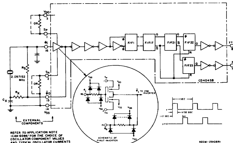
Fig. 1 - CD4045B and outboard components in a typical 21-stage counter application.
