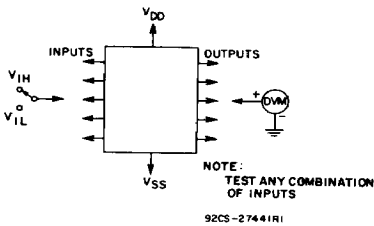
Fig. 13 - Noise-immunity test circuit.
