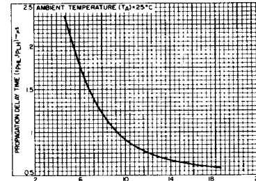
Fig. 6 - Typical propagation delay time as a function of supply voltage ( \phi_1 to y or y+d out vs. V_{DD} ).
