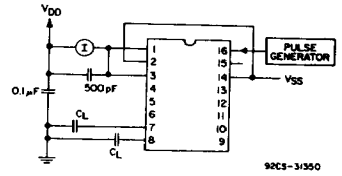
Fig. 15 - Dynamic power dissipation test circuit.
