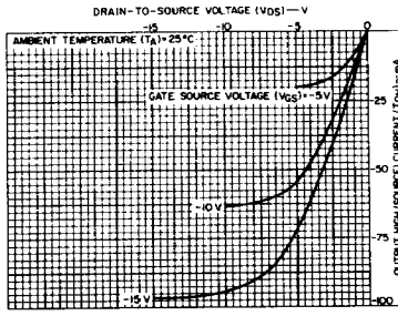
Fig. 5 - Minimum output high (source) characteristics.
