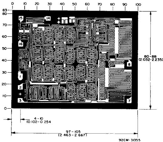
Dimensions and pad layout for CD4045B.
