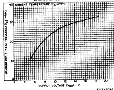
Fig. 8 - Typical maximum input-pulse frequency as a function of supply voltage.
