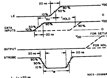
Fig. 14 - Dynamic waveforms.
