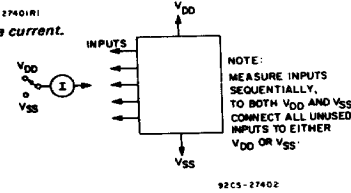
Fig. 11 - Input current.
