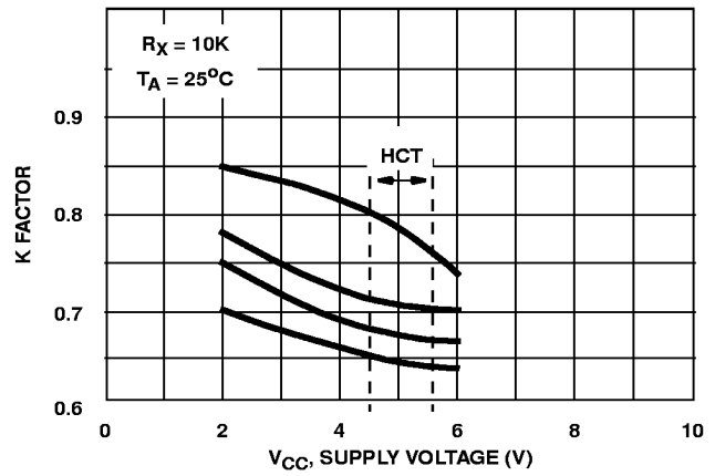
FIGURE 6. HC/HCT221 K FACTOR vs SUPPLY VOLTAGE
