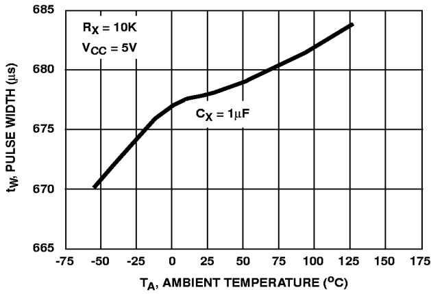
FIGURE 5. HC/HCT221 OUTPUT PULSE WIDTH vs TEMPERATURE
