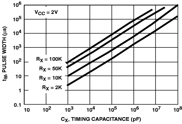
FIGURE 7. HC221 OUTPUT PULSE WIDTH vs C_X
