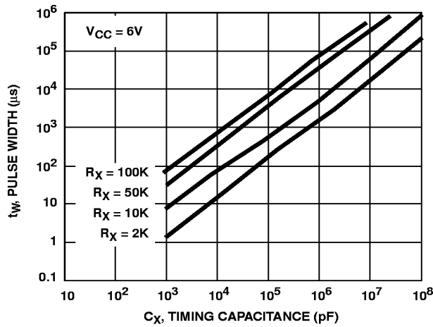
FIGURE 9. HC221 OUTPUT PULSE WIDTH vs C_X
