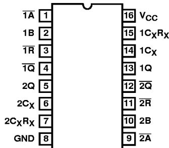
CD74HC221, CD74HCT221 (PDIP, SOIC) TOP VIEW
