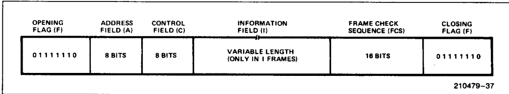
Figure 4. Frame Format
