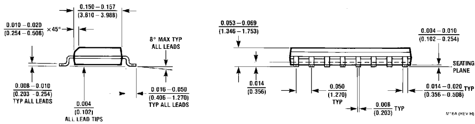
16-Lead Small Outline Molded Package (M) Order Number DM74LS174M or DM74LS175M NS Package Number M16A
