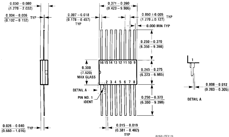
16-Lead Ceramic Flat Package (W) Order Number 54LS174FMQB, 54LS175FMQB, DM54LS174W or DM54LS175W NS Package Number W16A
