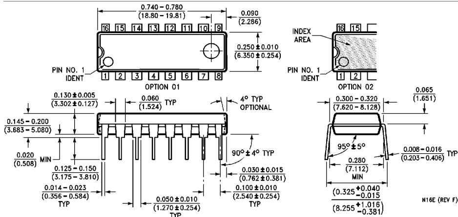
16-Lead Molded Dual-In-Line Package (N) Order Number DM74LS174N or DM74LS175N NS Package Number N16E
