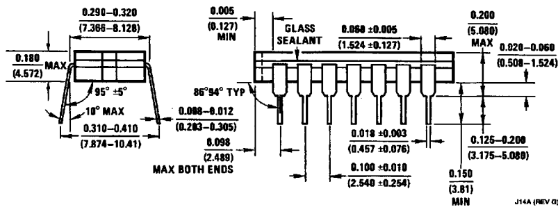
14-Lead Ceramic Dual-In-Line Package (J) Order Number DM54LS27J NS Package Number J14A
