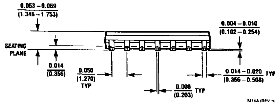
14-Lead Small Outline Molded Package (M) Order Number DM74LS27M NS Package Number M14A
