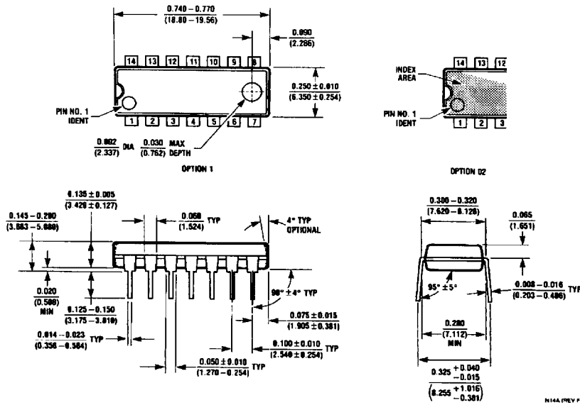
14-Lead Molded Dual-In-Line Package (N) Order Number DM74LS37N NS Package Number N14A
