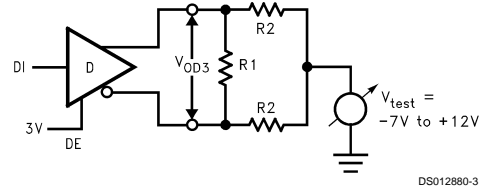
FIGURE 5. V_{OD3}
