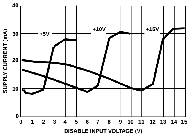
FIGURE 33. SUPPLY CURRENT vs DISABLE INPUT VOLTAGE
