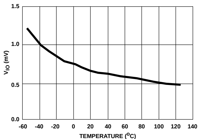
FIGURE 27. INPUT OFFSET VOLTAGE vs TEMPERATURE
