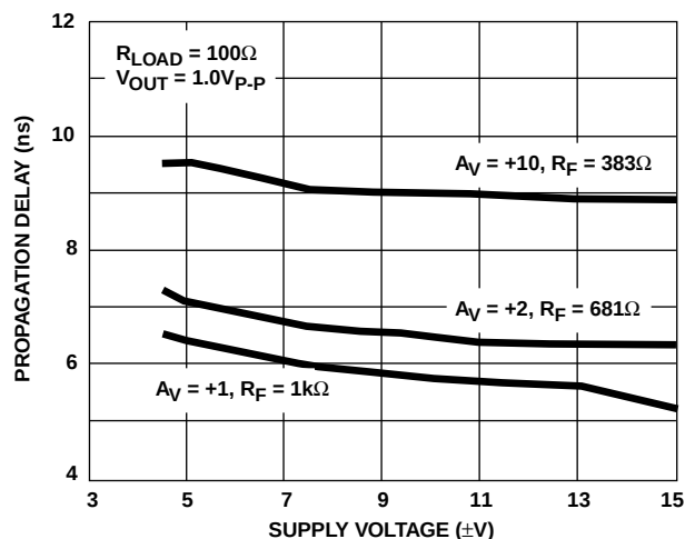
FIGURE 22. PROPAGATION DELAY vs SUPPLY VOLTAGE
