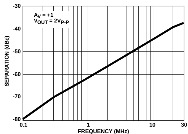
FIGURE 39. CHANNEL SEPARATION vs FREQUENCY
