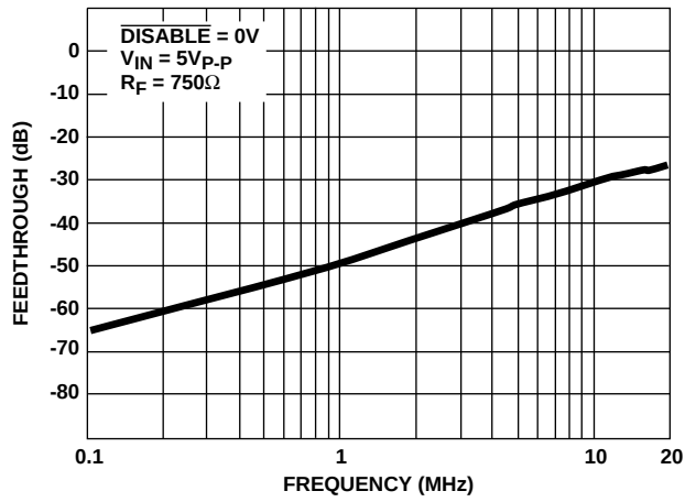
FIGURE 41. DISABLE FEEDTHROUGH vs FREQUENCY
