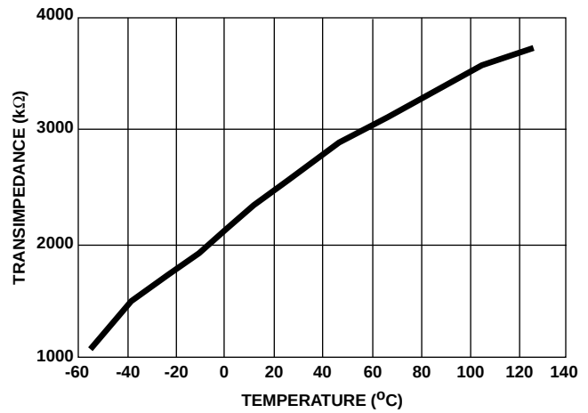
FIGURE 30. TRANSIMPEDANCE vs TEMPERATURE
