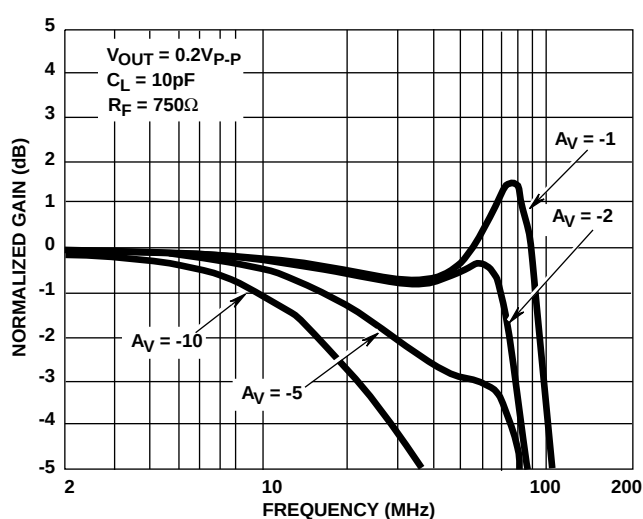
FIGURE 10. INVERTING FREQUENCY RESPONSE
