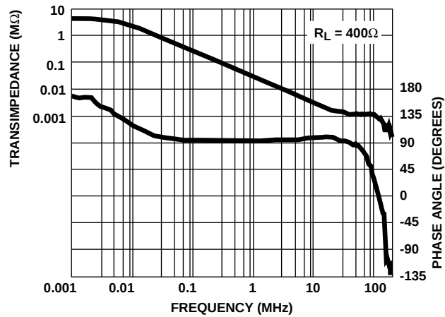
FIGURE 43. TRANSIMPEDANCE vs FREQUENCY
