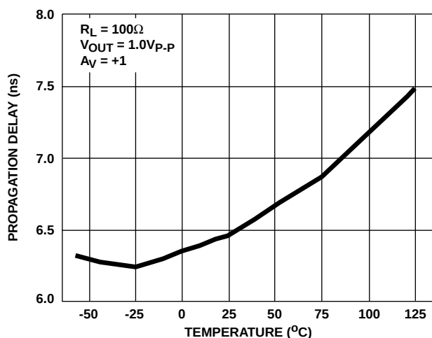
FIGURE 21. PROPAGATION DELAY vs TEMPERATURE
