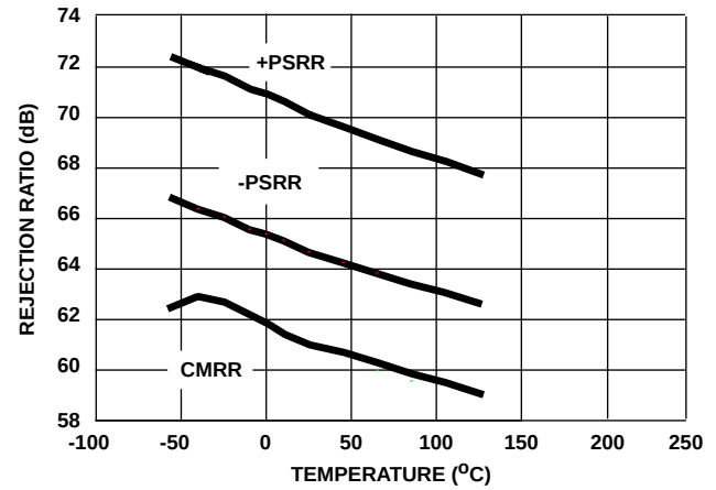
FIGURE 32. REJECTION RATIO vs TEMPERATURE
