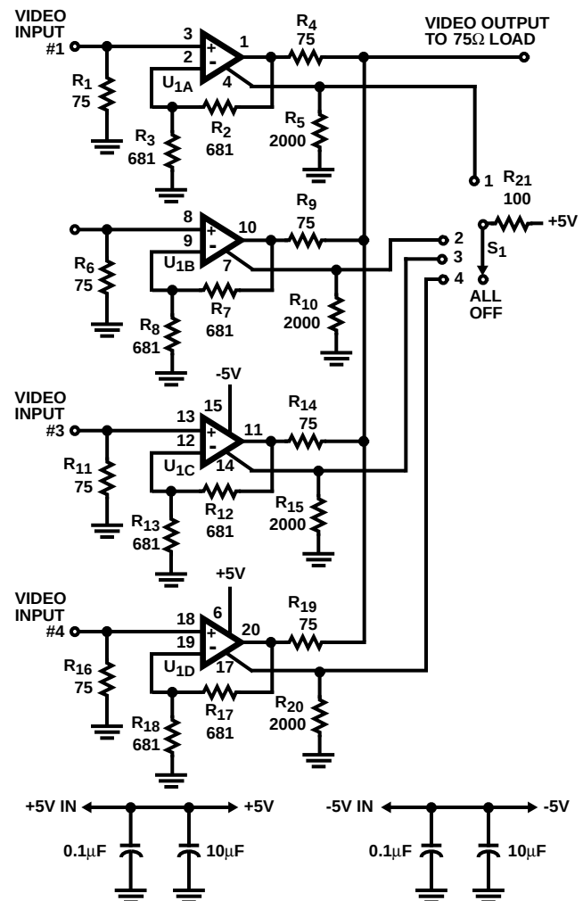
FIGURE 8. SIMPLIFIED SCHEMATIC OF ENABLE/DISABLE FUNCTION
