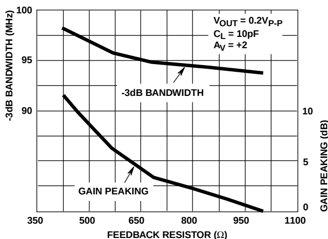
FIGURE 13. BANDWIDTH AND GAIN PEAKING vs FEEDBACK RESISTANCE
