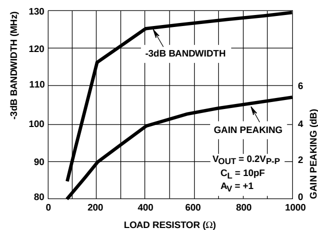
FIGURE 14. BANDWIDTH AND GAIN PEAKING vs LOAD RESISTANCE
