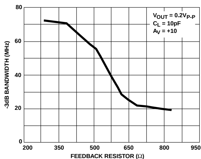
FIGURE 15. BANDWIDTH vs FEEDBACK RESISTANCE
