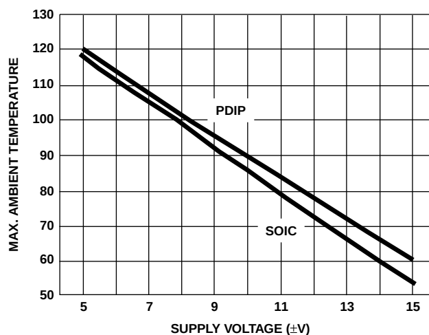
FIGURE 7. MAXIMUM OPERATING AMBIENT TEMPERATURE vs SUPPLY VOLTAGE
