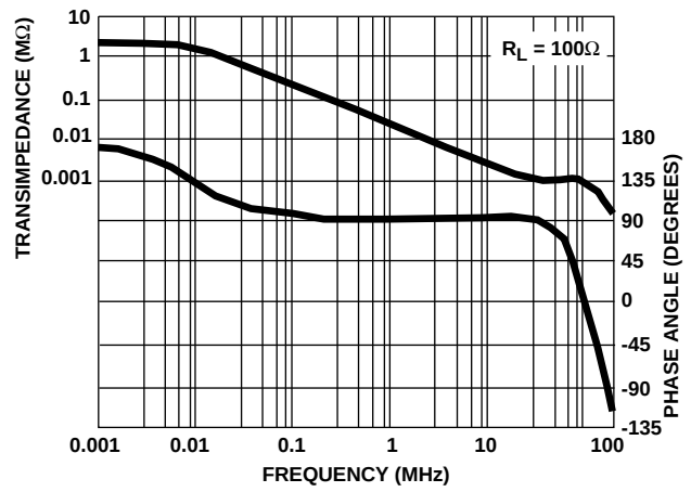
FIGURE 42. TRANSIMPEDANCE vs FREQUENCY
