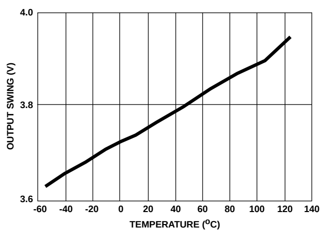
FIGURE 34. OUTPUT SWING vs TEMPERATURE
