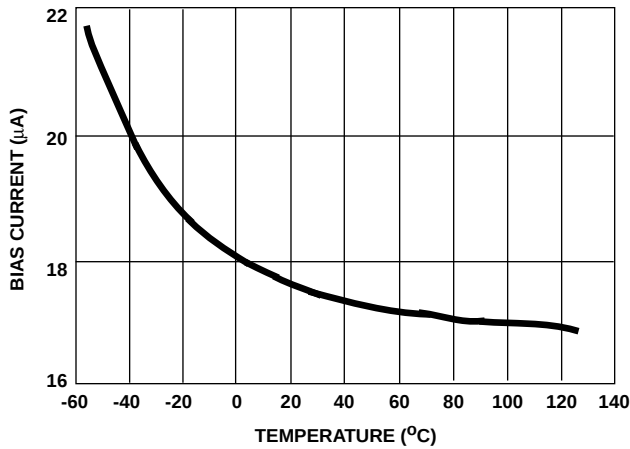
FIGURE 29. -INPUT BIAS CURRENT vs TEMPERATURE
