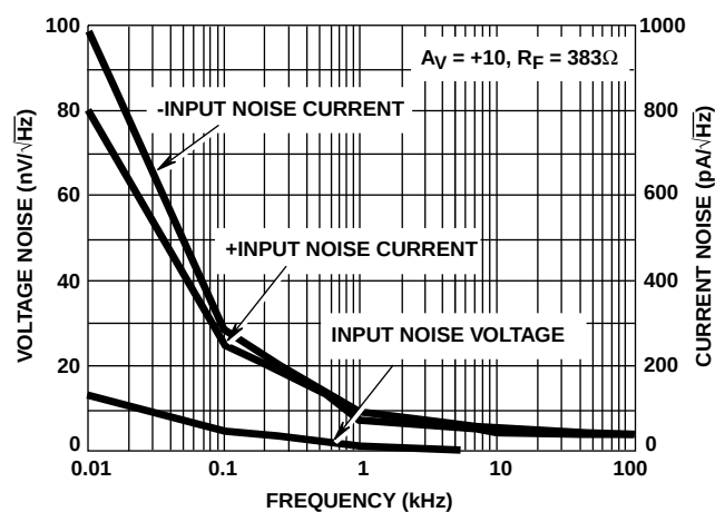
FIGURE 26. INPUT NOISE CHARACTERISTICS
