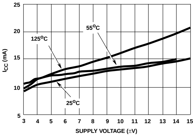
FIGURE 31. SUPPLY CURRENT vs SUPPLY VOLTAGE
