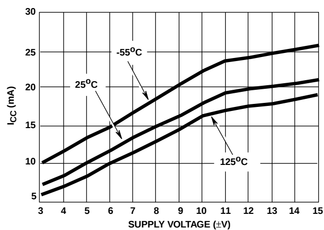
FIGURE 38. DISABLE SUPPLY CURRENT vs SUPPLY VOLTAGE
