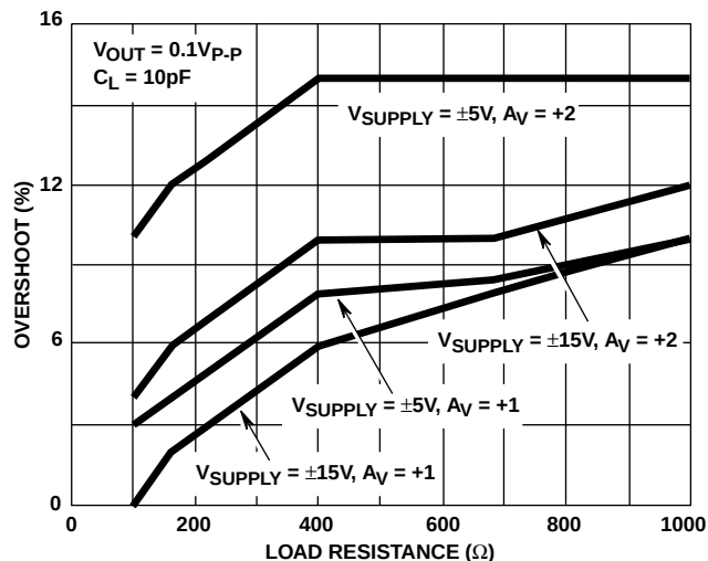
FIGURE 16. SMALL SIGNAL OVERSHOOT vs LOAD RESISTANCE
