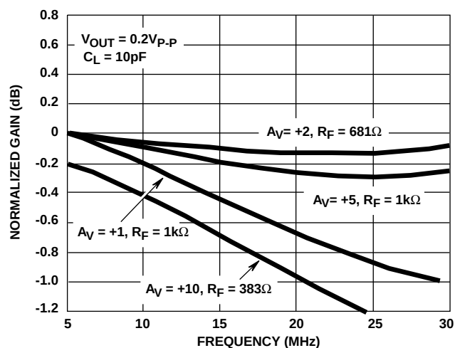
FIGURE 24. NON-INVERTING GAIN FLATNESS vs FREQUENCY
