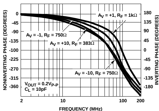
FIGURE 11. PHASE RESPONSE AS A FUNCTION OF FREQUENCY
