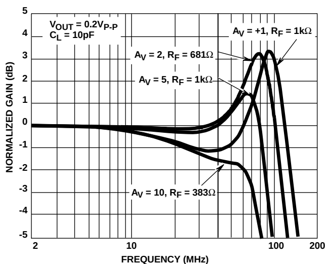
FIGURE 9. NON-INVERTING FREQUENCY RESPONSE
