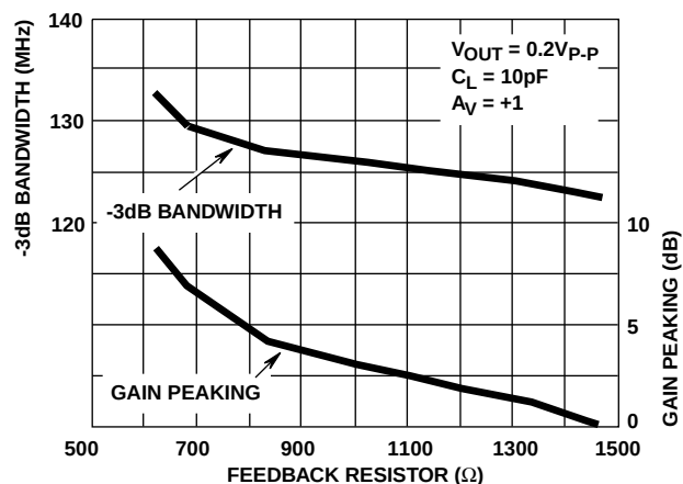
FIGURE 12. BANDWIDTH AND GAIN PEAKING vs FEEDBACK RESISTANCE
