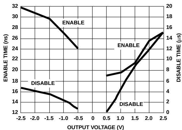
FIGURE 40. ENABLE/DISABLE TIME vs OUTPUT VOLTAGE
