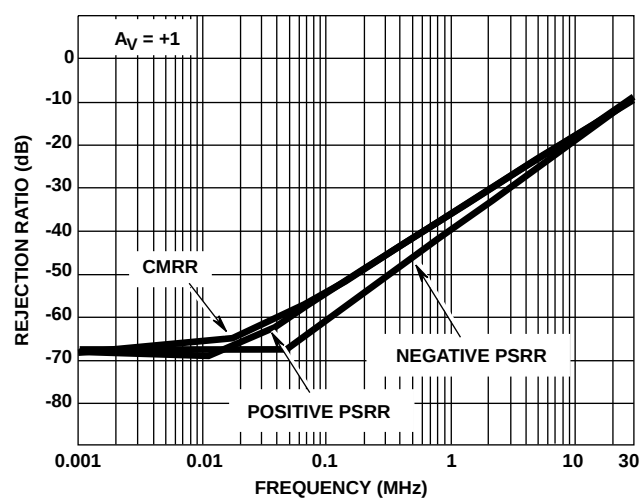
FIGURE 20. REJECTION RATIOS vs FREQUENCY
