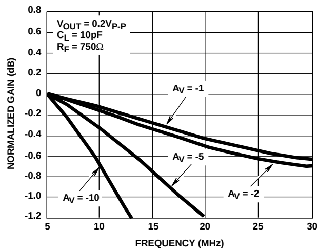
FIGURE 25. INVERTING GAIN FLATNESS vs FREQUENCY
