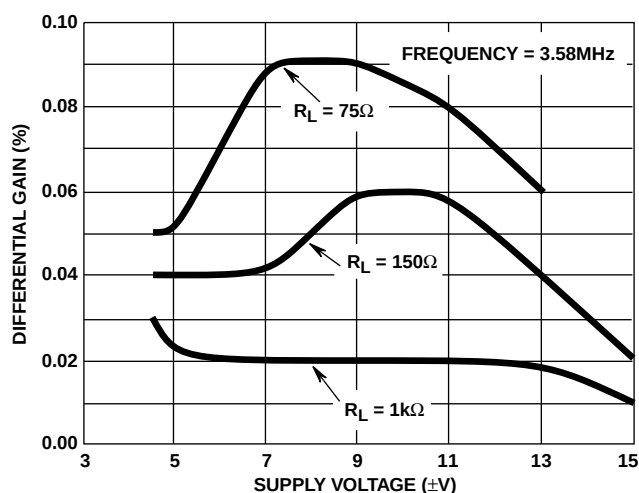
FIGURE 17. DIFFERENTIAL GAIN vs SUPPLY VOLTAGE
