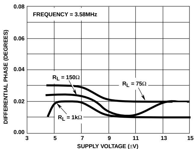
FIGURE 18. DIFFERENTIAL PHASE vs SUPPLY VOLTAGE
