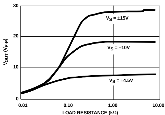
FIGURE 35. OUTPUT SWING vs LOAD RESISTANCE
