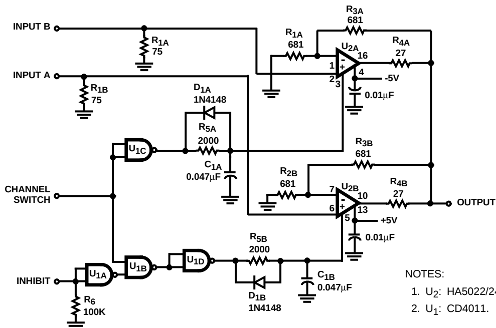
FIGURE 9. LOW IMPEDANCE MULTIPLEXER
