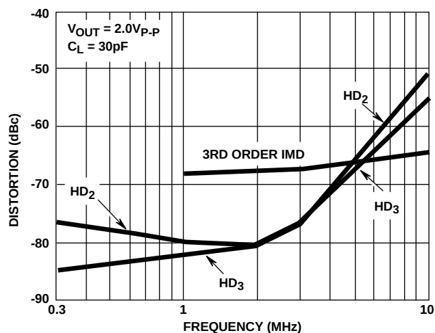
FIGURE 19. DISTORTION vs FREQUENCY
