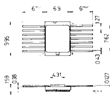
Ceramic flat package for HCC 4XXX BK
