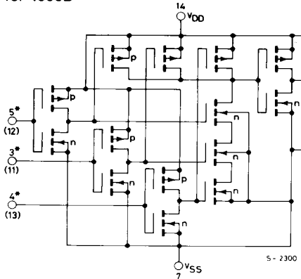
INVERTER AND 1 OF 2 GATES (NUMBERS IN PARENTHESES ARE TERMINAL NUMBERS FOR SECOND GATE)
