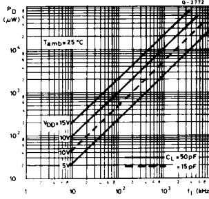
Typical power dissipation per gate vs. frequency
