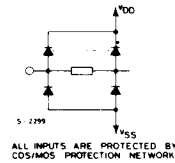
ALL INPUTS ARE PROTECTED BY COS/MOS PROTECTION NETWORK
