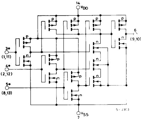
INVERTER AND 1 OF 3 GATES (NUMBERS IN PARENTHESES ARE TERMINAL NUMBERS FOR SECOND GATE)
