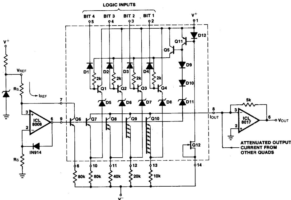
Figure 4: Typical Circuit
