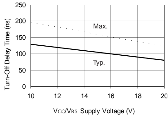
Figure 8B. Turn-Off Time vs. V cc /V s Supply Voltage
