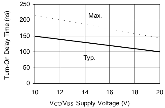
Figure 7B. Turn-On Time vs. V cc /V s Supply Voltage
