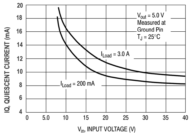
Figure 6. Quiescent Current
