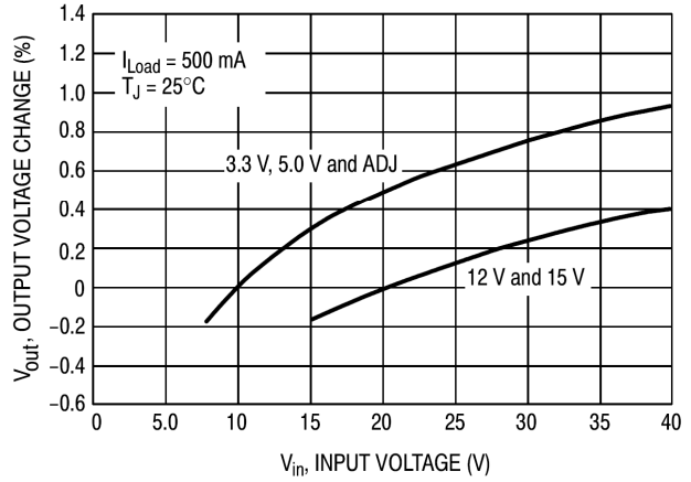
Figure 3. Line Regulation
