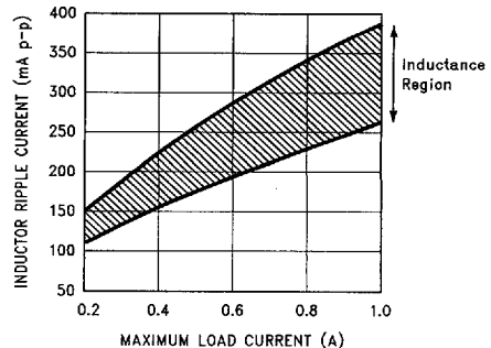
FIGURE 18. Peak-to-Peak Inductor Ripple Current vs Load Current
