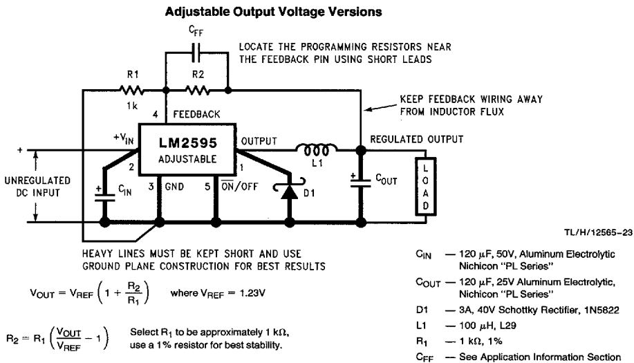
FIGURE 2. Standard Test Circuits and Layout Guides
