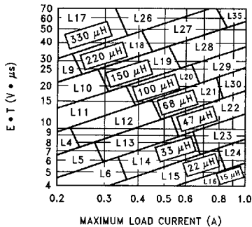
FIGURE 8. LM2595-ADJ
