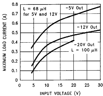
FIGURE 26. Inverting Regulator Typical Load Current
