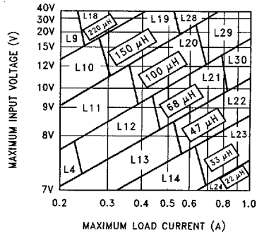
FIGURE 6. LM2595-5.0
