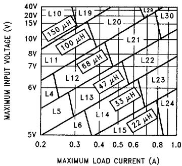
FIGURE 5. LM2595-3.3
