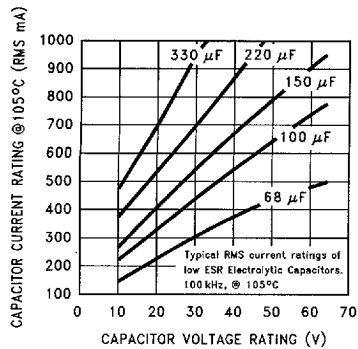
FIGURE 13. RMS Current Ratings for Low ESR Electrolytic Capacitors (Typical)
