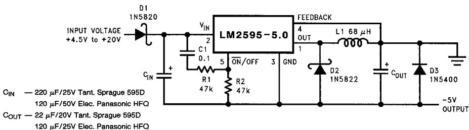
FIGURE 25. Inverting -5V Regulator with Delayed Startup
