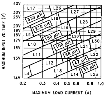
FIGURE 7. LM2595-12
