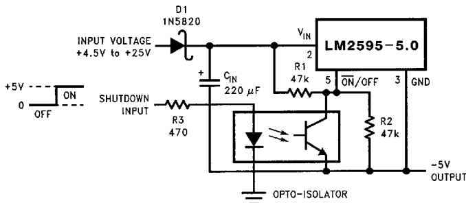
FIGURE 28. Inverting Regulator Ground Referenced Shutdown using Opto Device
