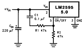
FIGURE 21. Delayed Startup
