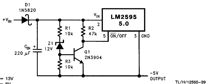
FIGURE 24. Undervoltage Lockout with Hysteresis for Inverting Regulator
