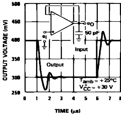
VOLTAGE FOLLOWER PULSE RESPONSE (SMALL SIGNAL)
