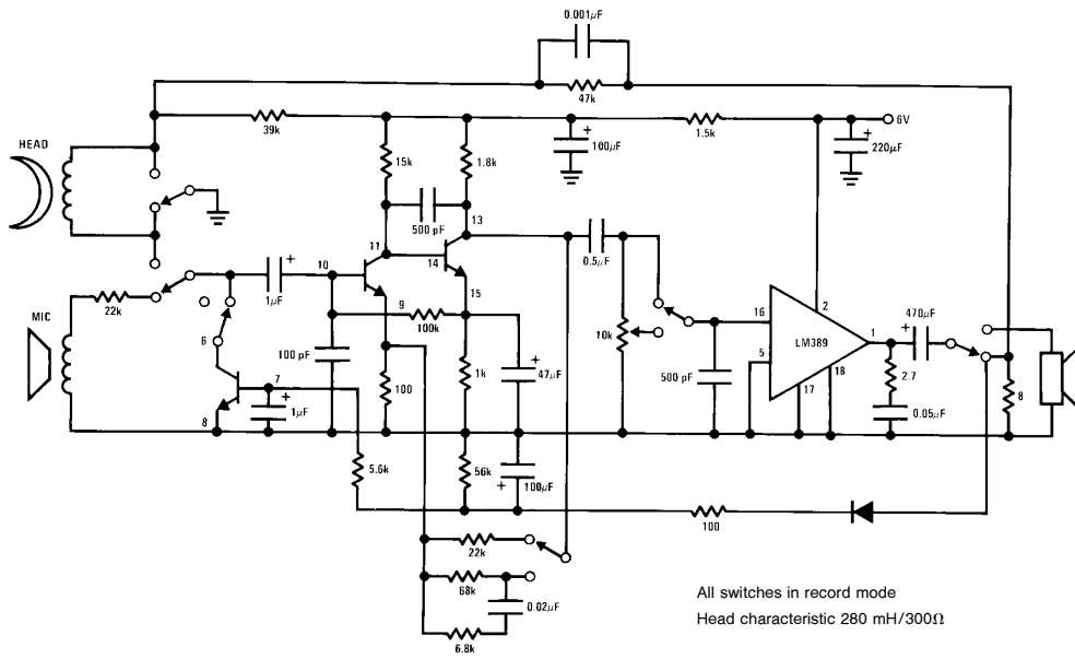
FIGURE 2. Tape Recorder
