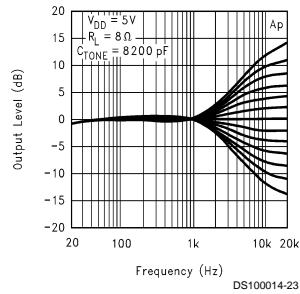
Treble Response vs Frequency
