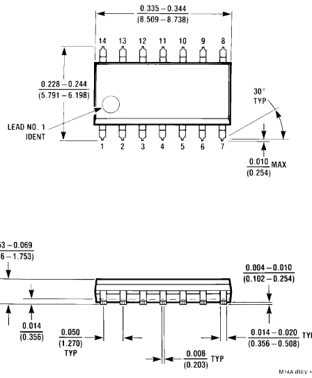
14-Pin Small Outline Package Order Number LM6144AIM or LM6144BIM NS Package Number M14A
