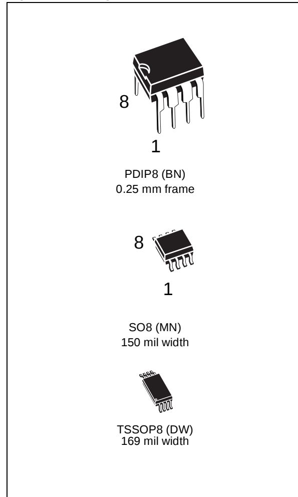
Figure 1. Packages
