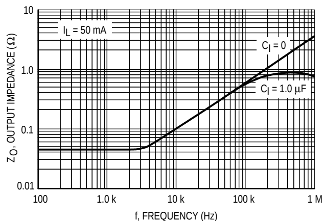
Figure 15. Output Impedance as Function of Frequency
