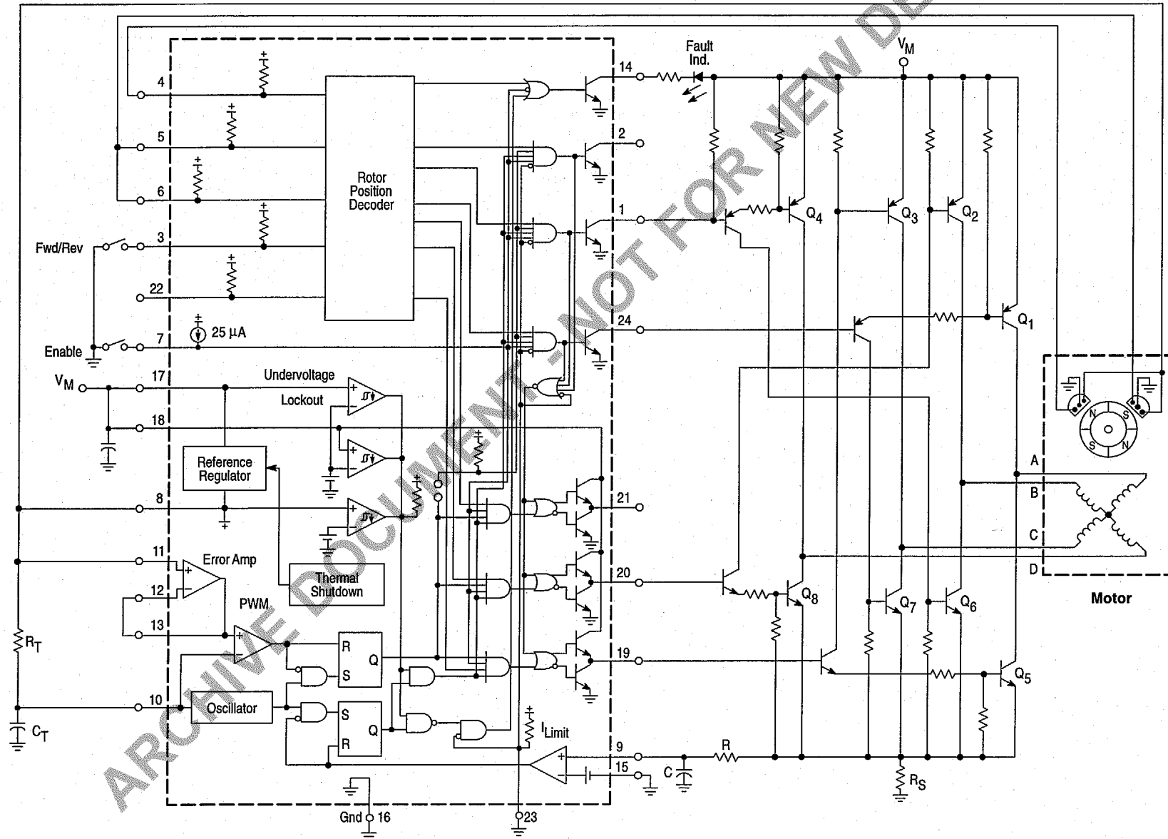
Figure 43. Four Phase, Four Step, Full Wave Motor Controller
