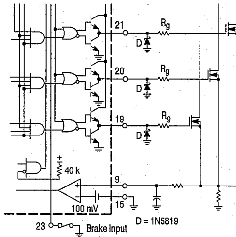
Figure 27. MOSFET Drive Precautions
