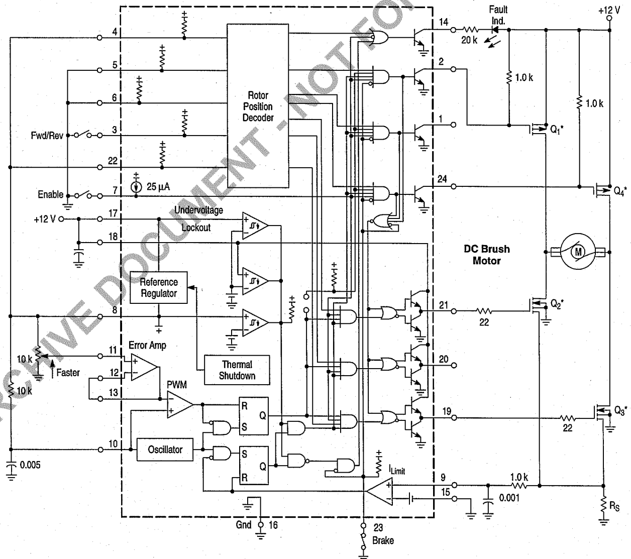
Figure 46. H-Bridge Brush-Type Controller
