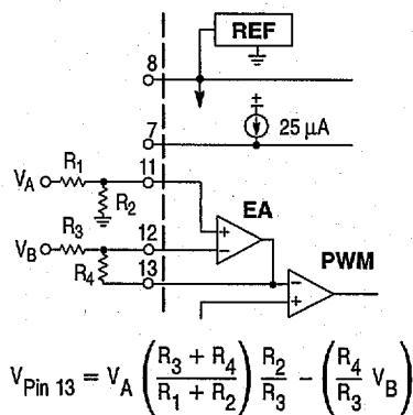
Figure 31. Differential Input Speed Controller
