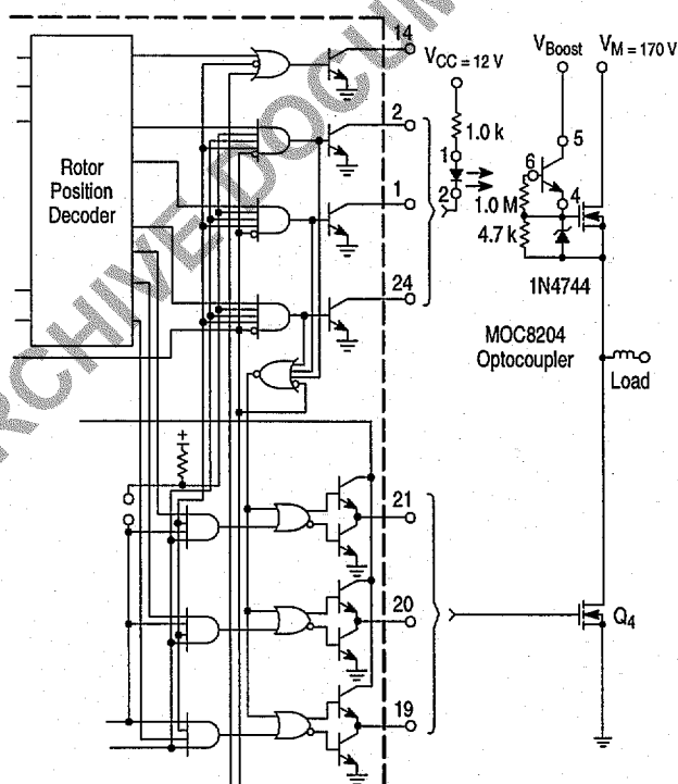
Figure 25. High Voltage Interface with N-Channel Power MOSFETs
