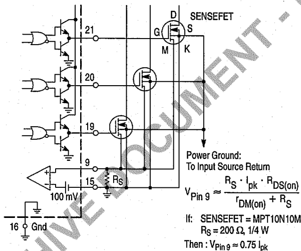
Figure 29. Current Sensing Power MOSFETs
