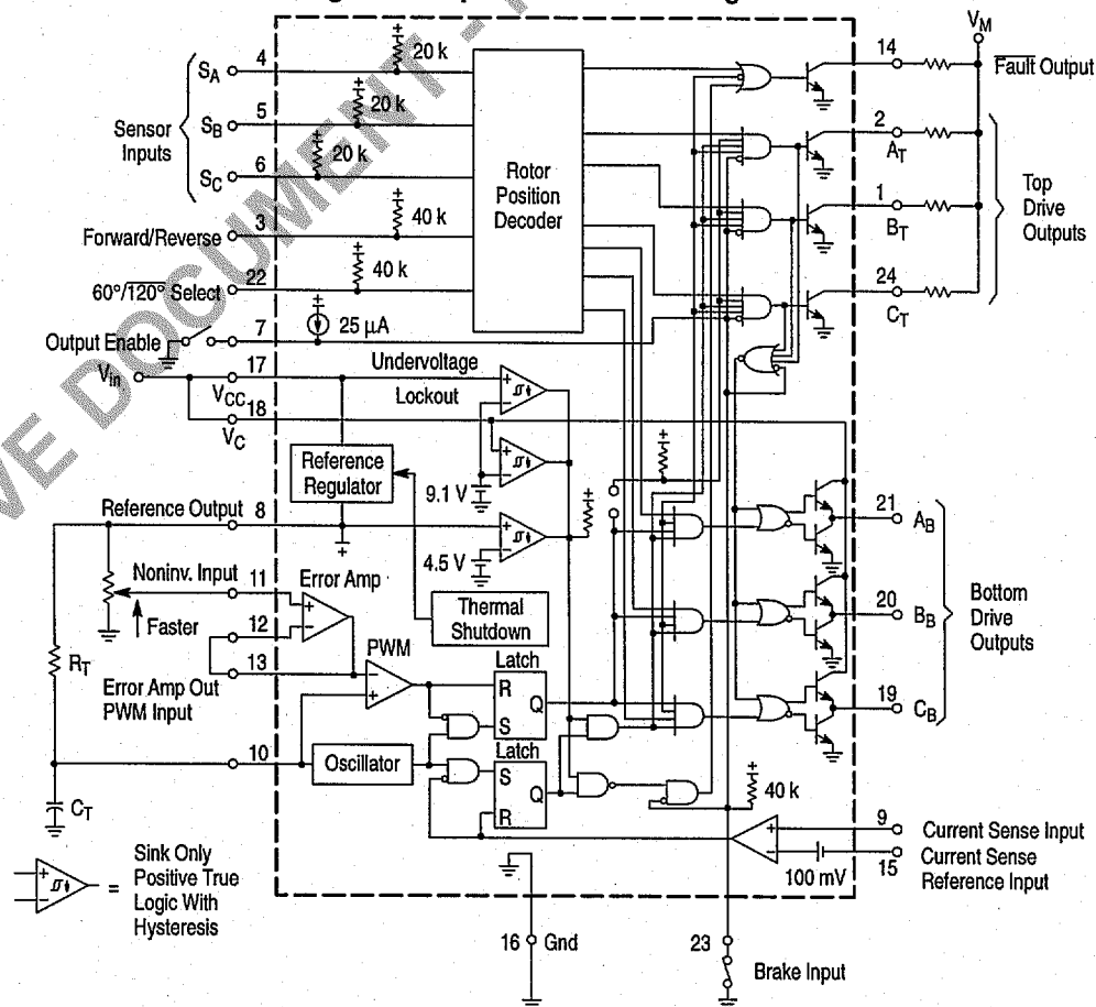
Figure 19. Representative Block Diagram
