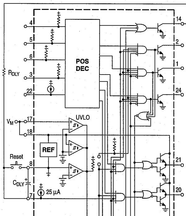
Figure 23. Timed Delayed Latched Over Current Shutdown
