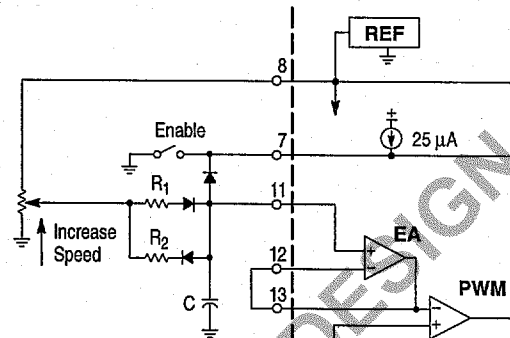
Figure 32. Controlled Acceleration/Deceleration
