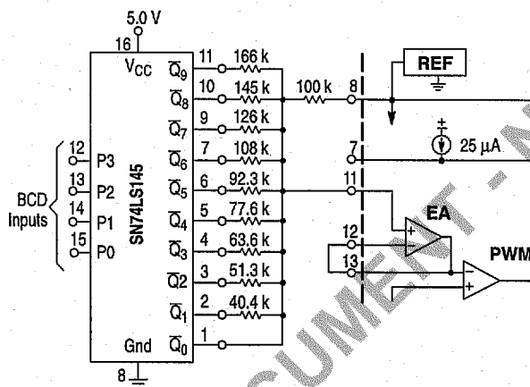
Figure 33. Digital Speed Controller
