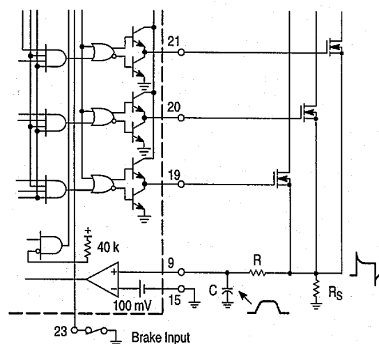
Figure 26. Current Waveform Spike Suppression
