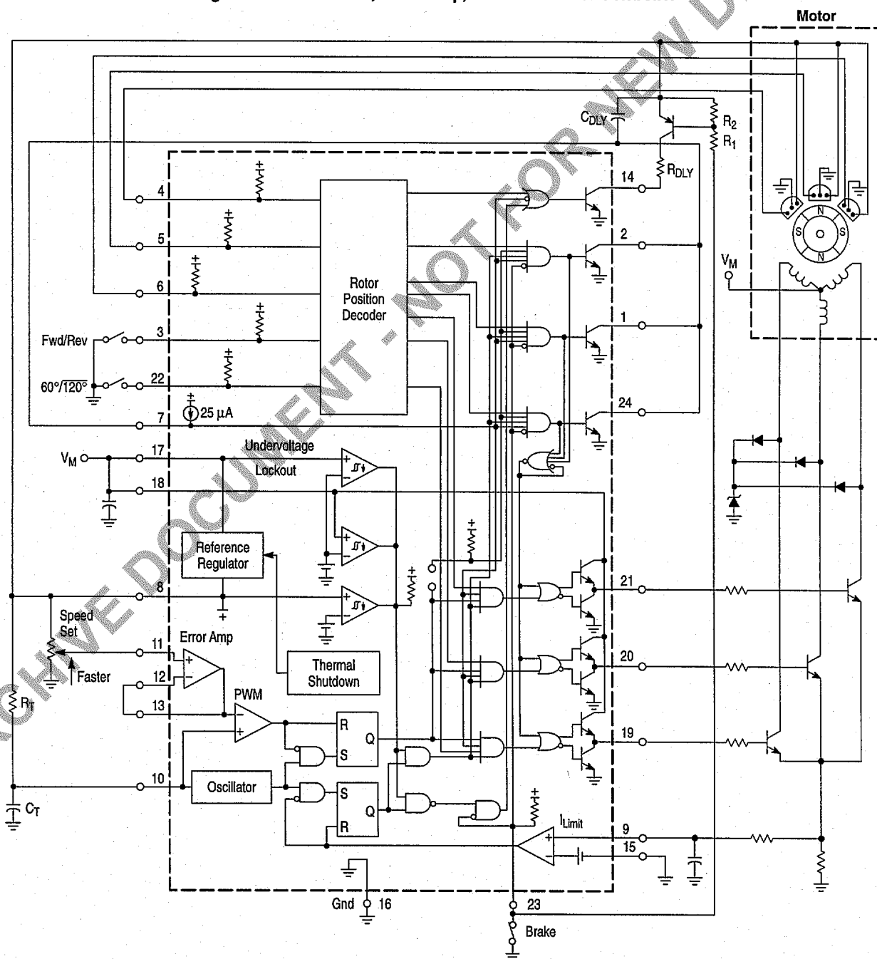
Figure 38. Three Phase, Three Step, Half Wave Motor Controller
