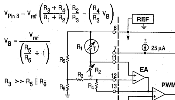
Figure 35. Closed Loop Temperature Control
