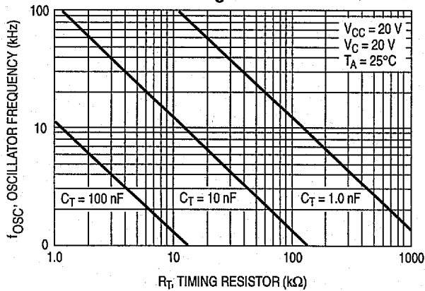
Figure 1. Oscillator Frequency versus Timing Resistor
