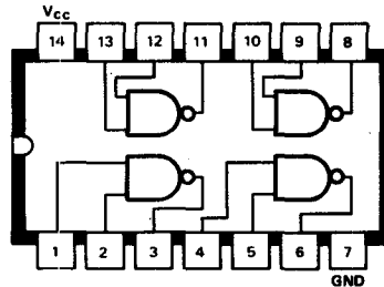
B30 SN7438N/AN Quad 2-input NAND Buffer with open collector output
