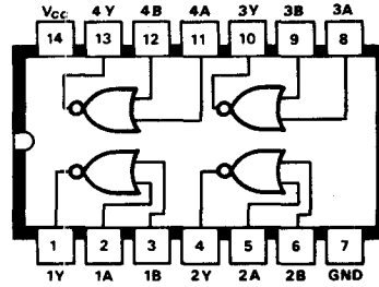
B28 SN7433N/AN Quad 2-input NOR Buffer with open collector output
