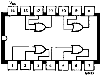
B27 SN7432N SN74S32N Quad 2-input OR gate
