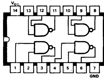
B29 SN7437N SN74S37N Quad 2-input NAND gate
