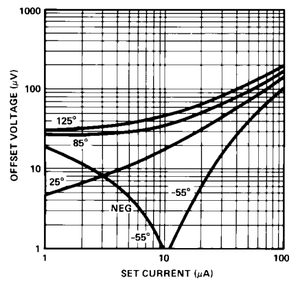
OFFSET VOLTAGE vs SET CURRENT
