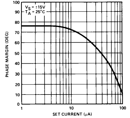
PHASE MARGIN vs SET CURRENT
