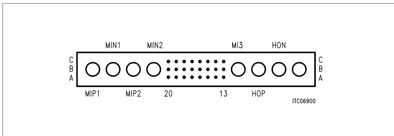
Figure 3 Pin-Outs of the Audio Interface Connector AIC
