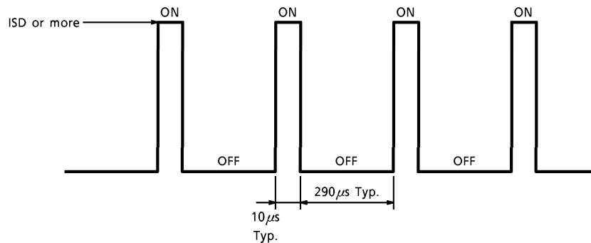
Figure 1 Switching Waveforms
