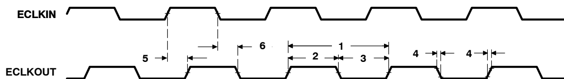
Figure 33. ECLKOUT Timings
