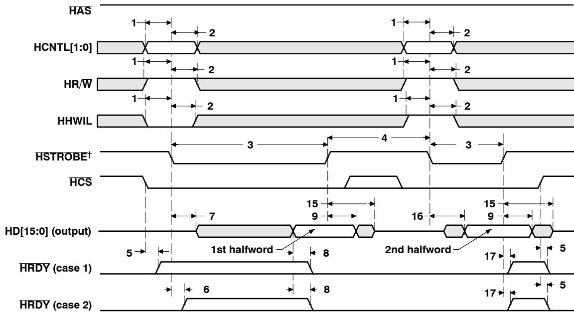
Figure 53. HPI Read Timing ( \overline{HAS} Not Used, Tied High)
