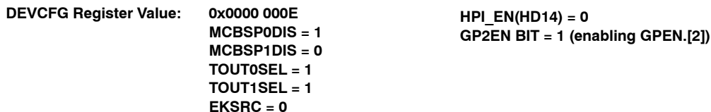
Figure 7. Configuration Example B (1 I2C + 1 McBSP + 2 McASP + GPIO)
