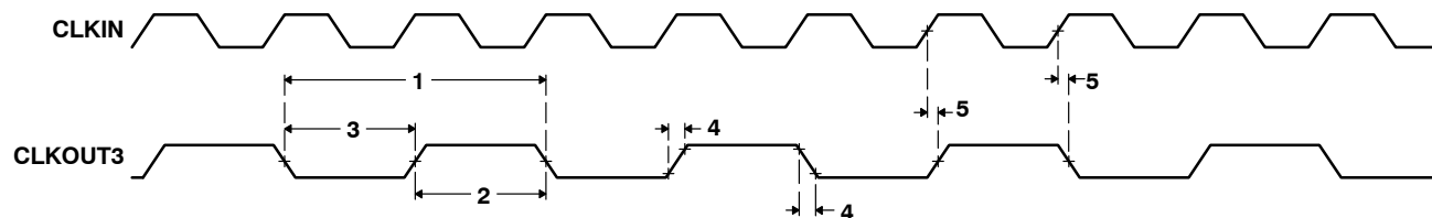
Figure 31. CLKOUT3 Timings
