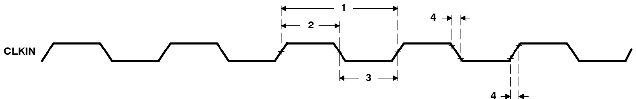
Figure 29. CLKIN Timings
