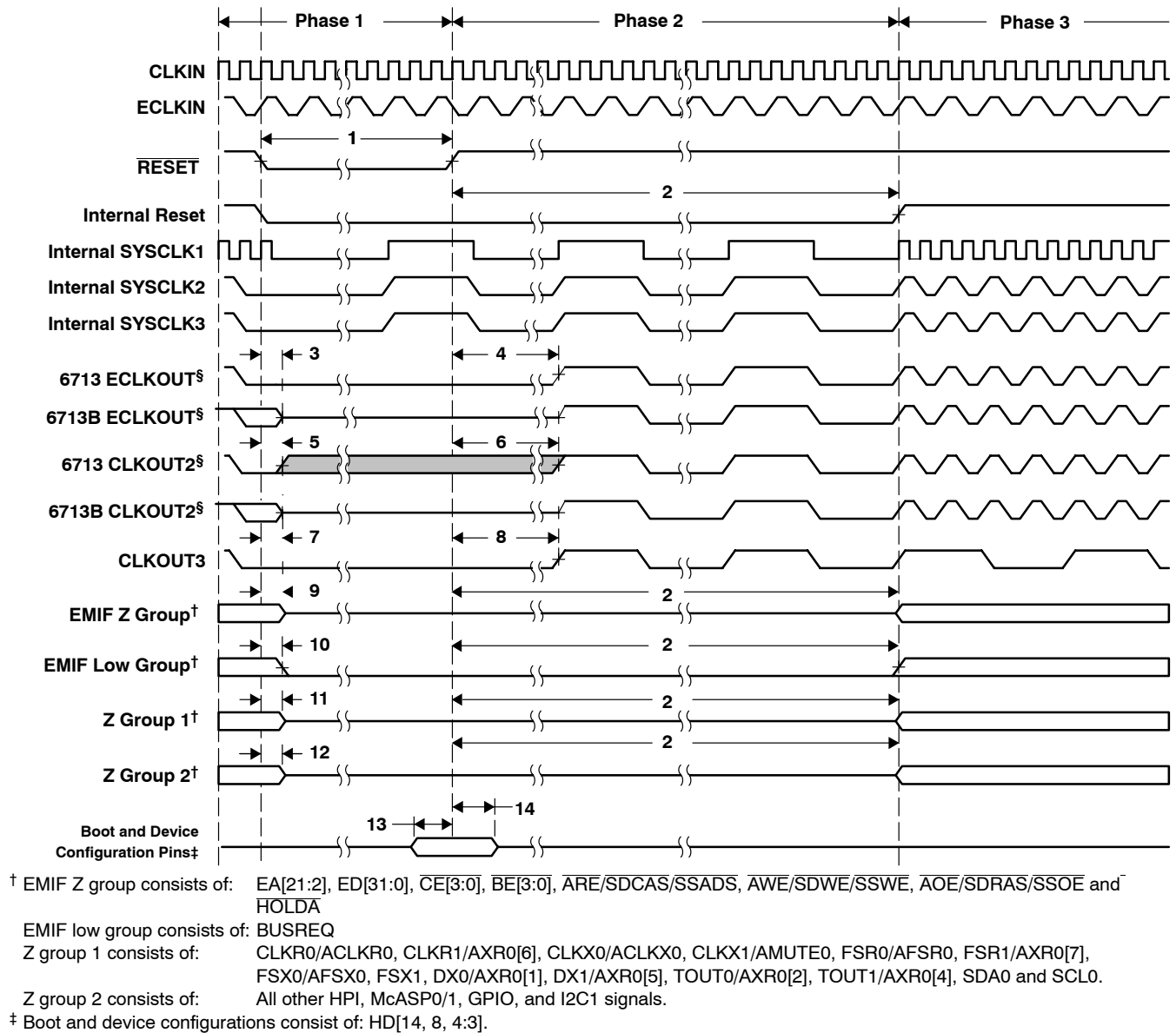
Figure 47. Reset Timing
