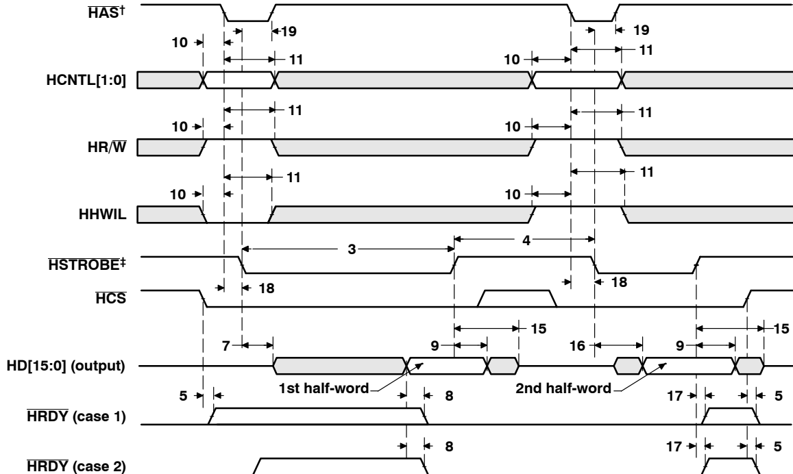
Figure 54. HPI Read Timing ( \overline{HAS} Used)
