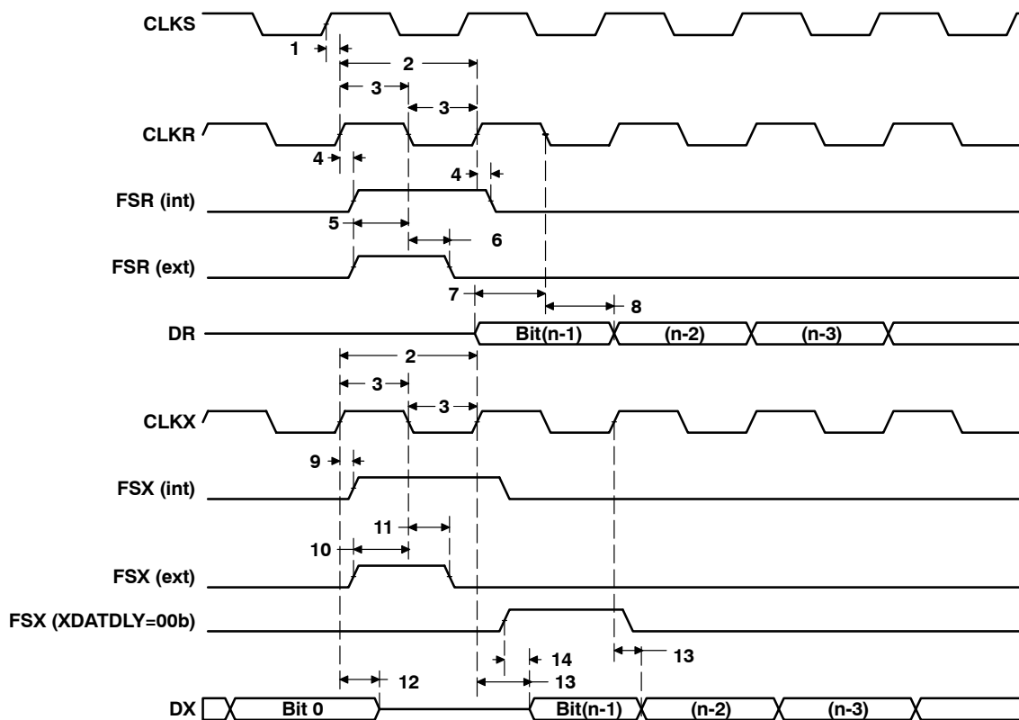
Figure 57. McBSP Timings
