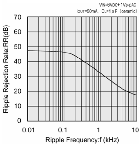
XC6202P502 (5.0V)
