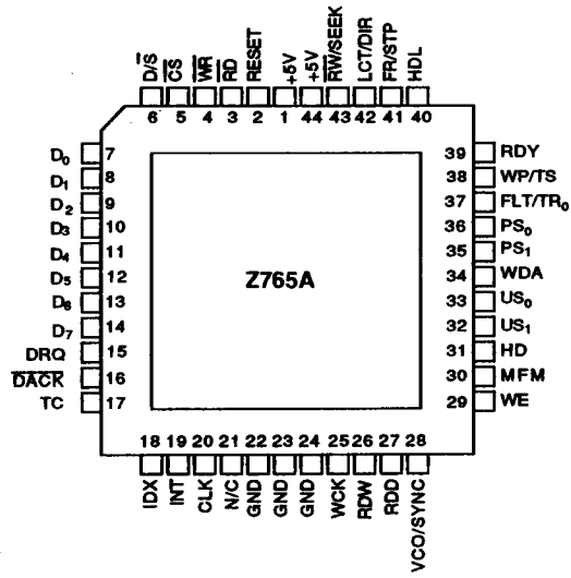
Figure 3b. Pin Assignments
