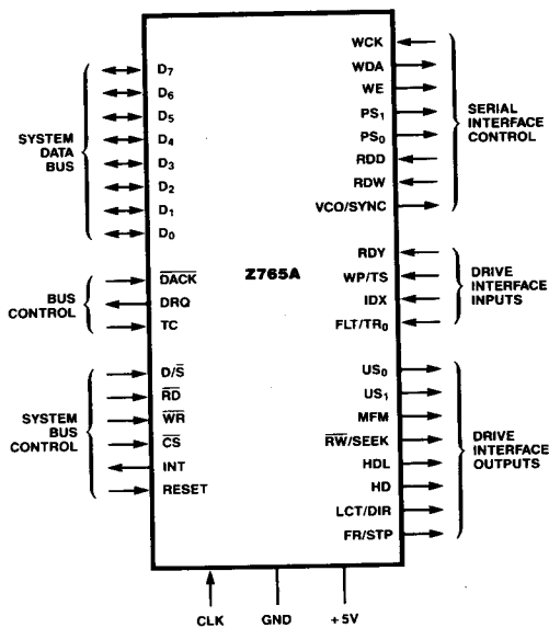
Figure 2. Pin Functions
