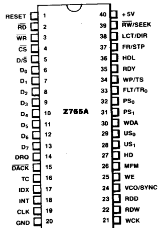
Figure 3a. Pin Assignments
