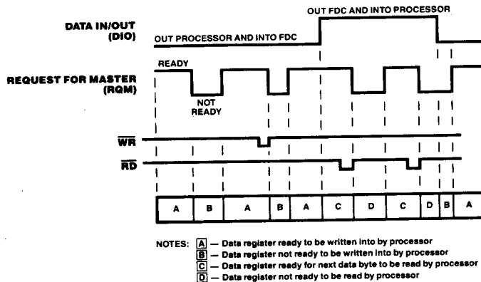
Figure 4. Data Transfer
