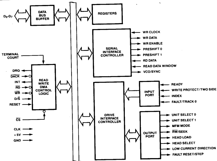
Figure 1. Z765A FDC Block Diagram
