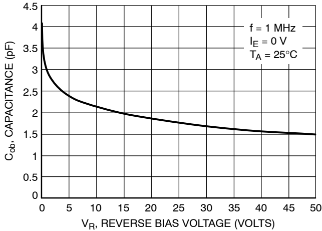
Figure 49. Output Capacitance
